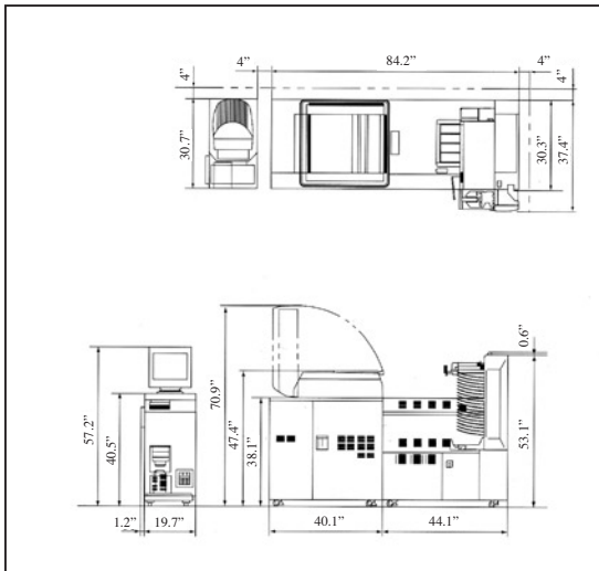
QSS-31 PRO External View
