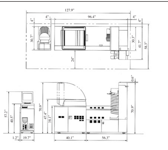
QSS-31 PRO TURBO External View
